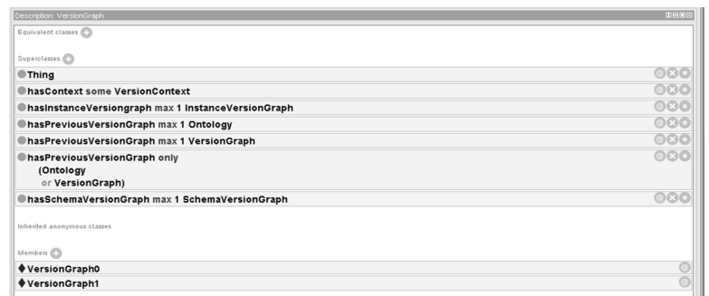
Figure 3. VersionGraph definition in Protege.
