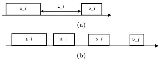
Fig. 1 A single coupled-task and two compatible coupled-tasks.
