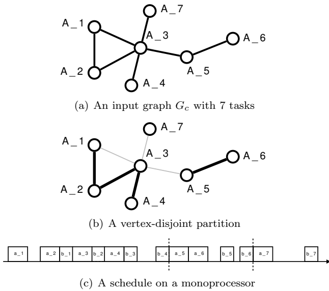
Fig. 3 Relation between a schedule and a partition into vertex-disjoint paths
