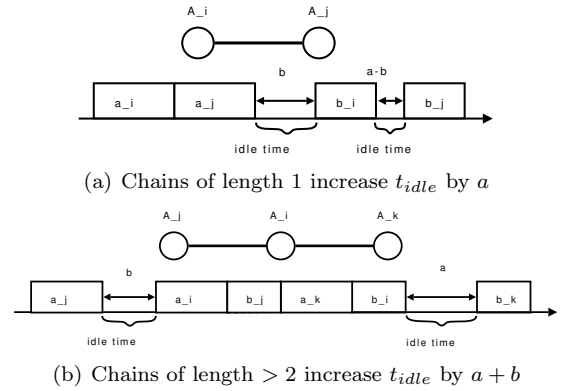
Fig. 4 Impact of the length of the paths on the idle time
