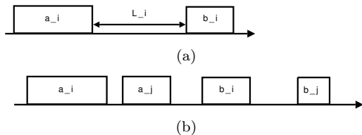
Fig. 1 A single coupled-task and two compatible coupled-tasks.
