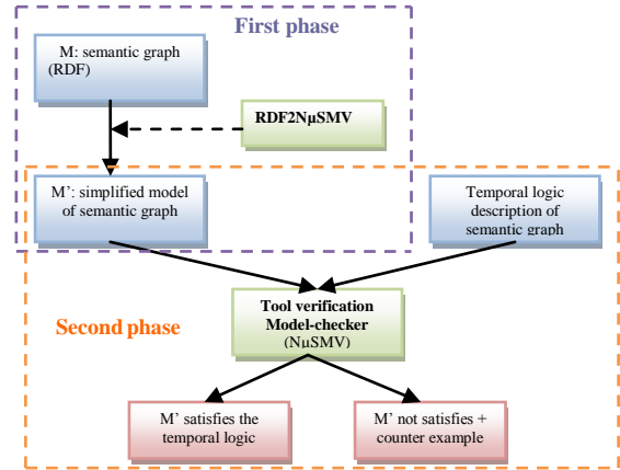
Figure 5. Our architecture.
