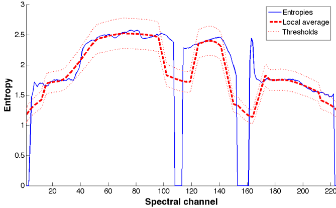
Figure 2. Exclusion of irrelevant bands: entropy, local average and thresholds for the "Jasper Ridge" image. Channels outside the rejection thresholds are excluded ( \delta = 10\% and s = 11 ).
