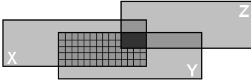
Figure 1. Venn representation of mutual information. The three rectangles depict the entropy of a random variable each. The overlappings represent the information shared by several variables. The squared area represents the conditional mutual information I(X; Y|Z) .
