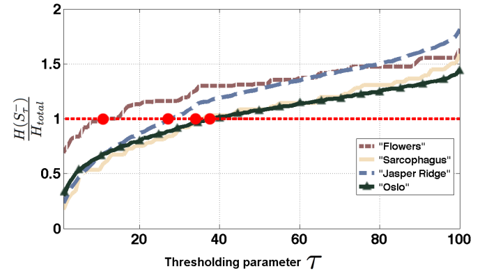
Figure 6. The proportion of discarded entropy in regards to \tau
