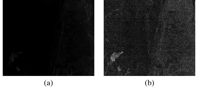
Figure 3. Example of excluded bands: (a) num 5 (b) num 164. The first one falls below the relevance range because of its very low mean value. The second one is rejected for it contains too much spatial noise.
