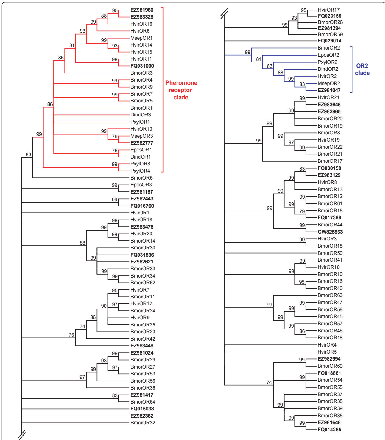
Figure 5 Phylogenetic tree of candidate olfactory receptors (ORs) from S. littoralis , B. mori and other lepidopterans, including pheromone receptor (PR) and OR2 ( D. melanogaster OR83b orthologue) clades. The S. littoralis translated unigenes are shown in bold. Accession numbers are given in additional file 6. The tree was constructed as in figure 4. Bmor, Bombyx mori ; Dind, Diaphania indica ; Epos, Epiphyas postvittana ; Hvir, Heliothis virescens ; Msep, Mythimna separata ; Pxyl, Plutella xylostella .
