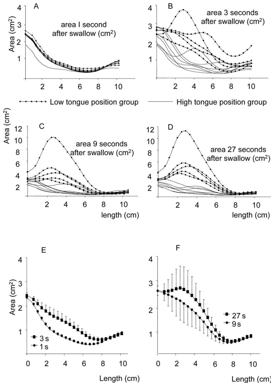
Figure 4. In-mouth air cavity cross-section as a function of the in-mouth air cavity, antero-posterior section level. A, B, C, D: Individual in-mouth air cavity cross-section (cm 2 ) at four times points (1, 3, 9 and 27 seconds) after swallowing ( n = 12). The two groups were identified in Experiment 1. After deglutition, one group displayed a large in-mouth air cavity (lines with dots), and another displayed a small in-mouth air cavity (lines without dots). E and F: Mean tongue position (mean cross section area ± standard error) of the 12 subjects at 1, 3, 9 and 27 s after swallowing. The subjects received no about the tongue position in the mouth, breathing or inter-arch contact. Monitoring showed that the subjects breathed through their noses.
