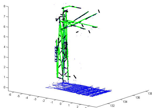
Figure 3: Mast detection
