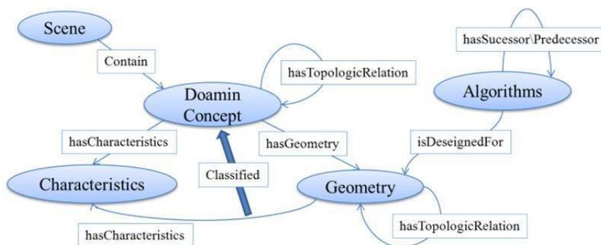
Fig. 7. Ontology general schema overview.
