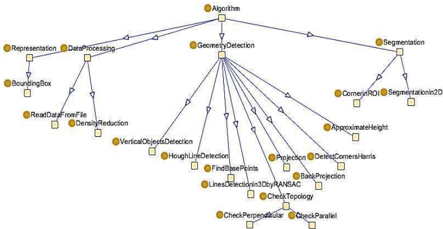
Fig. 12. Hierarchical structure of the Algorithm class.
