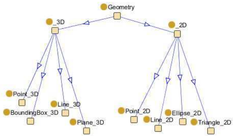
Fig. 9. The geometry class hierarchy.
