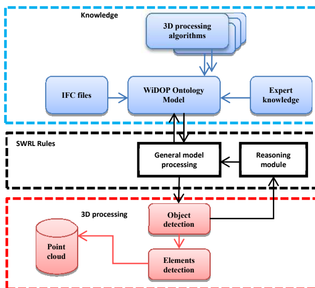
Fig. 5. WiDOP: Overview system.
