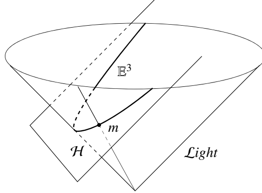
Figure 3: Euclidean models in the Lorentz space \mathbb{R}^5_1 .
