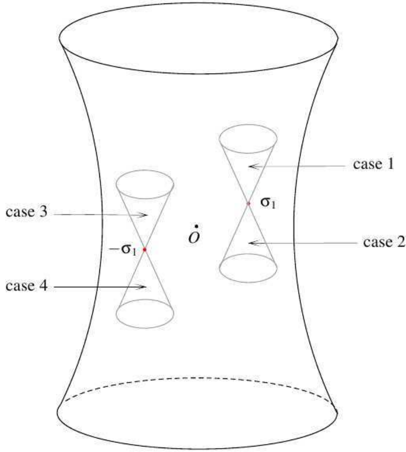
Figure 5: The two cones C_{\sigma_1} and C_{-\sigma_1} . Case 1: B_1 \cap B_2 = B_2 . Case 2: B_1 \cap B_2 = B_1 . Case 3: B_1 \cap B_2 = \emptyset . Case 4: B_1 \cap B_2 \simeq \mathbb{S}^2 \times [0, 1] .
