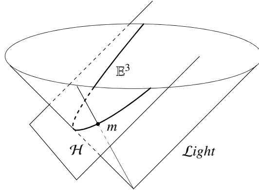
Figure 3: Euclidean models in the Lorentz space \mathbb{R}_1^5 .
