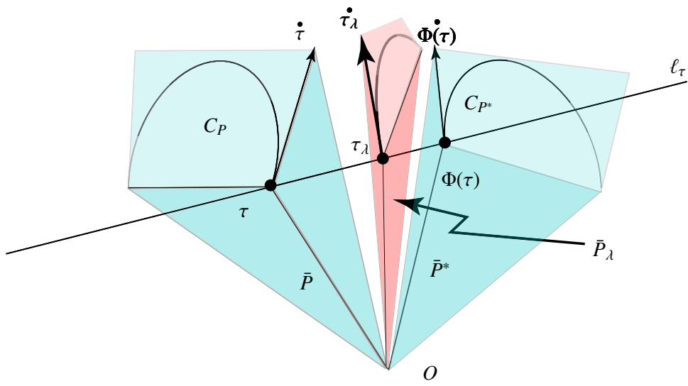
Figure 26: Orthogonal spaces \bar{P}, \bar{P}^* in \mathbb{R}_2^6 and a subspace \tilde{P}_\lambda \subset \mathbb{R}_2^6
