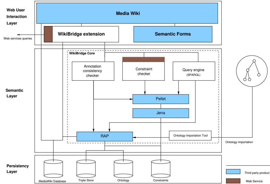
Fig. 2. WikiBridge's Architecture
