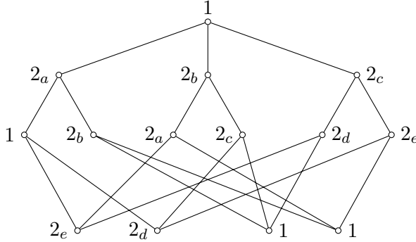
Figure 5: A cubic bipartite (1, 2, 2, 2, 2, 2) -chromatic graph of order 14.
