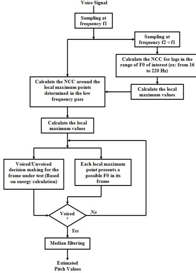
Fig. 5. Pitch tracking
