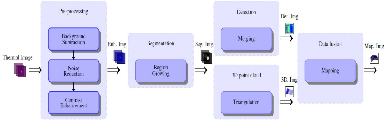
Fig. 2. Algorithm work flow.
