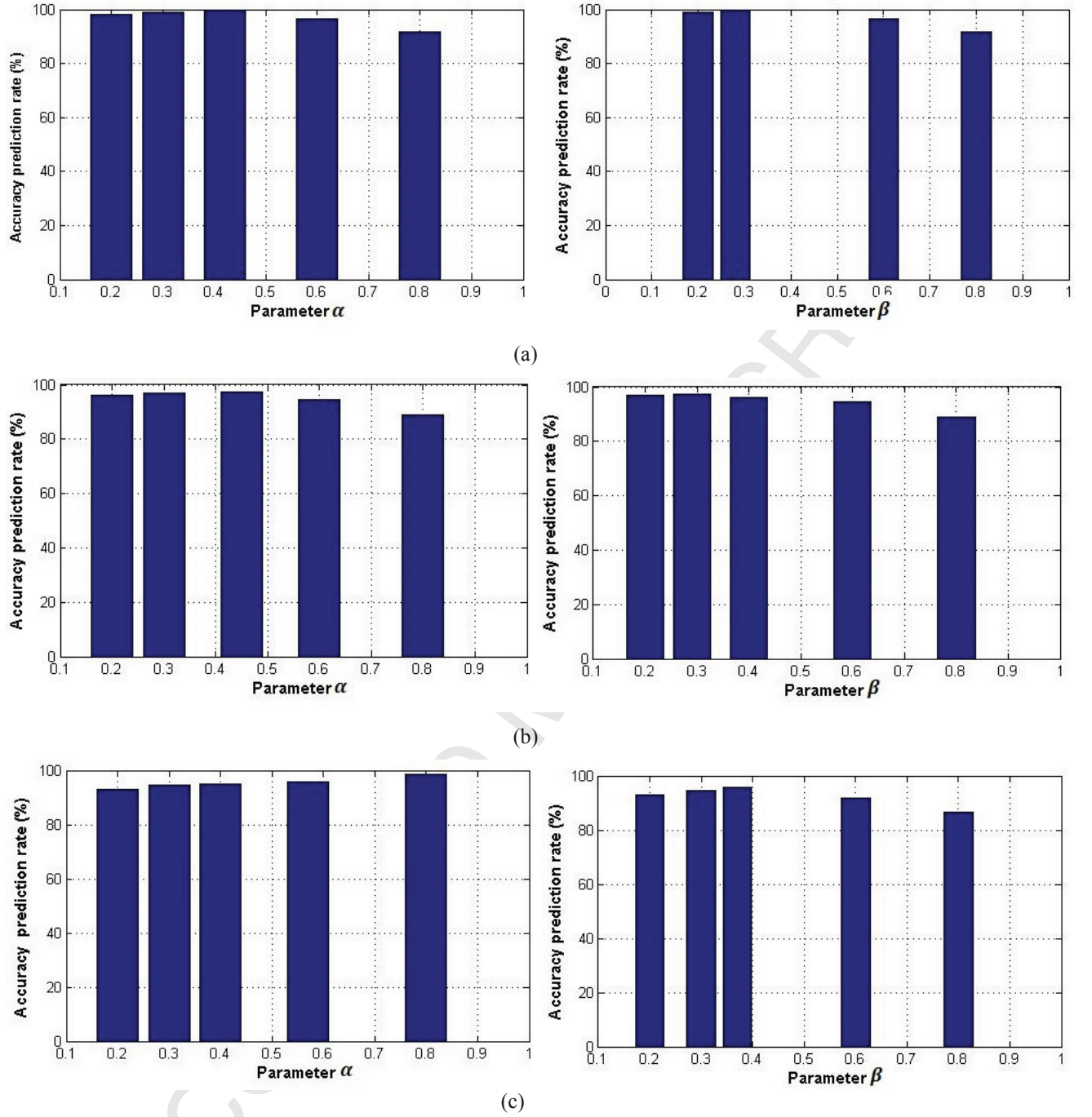
Fig.4 Optimal probability thresholds with a number of attackers equal to (a) 10%, (b) 20% and (c) 40 % of overall vehicles.
