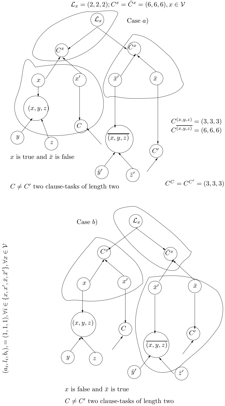
FIGURE 2. A partial compatibility graph for the \mathcal{NP} -completeness of the scheduling problem 1|\alpha(t_i), G = 1\text{-stage bipartite}, d_G(X) = 2, d_G(Y) \in \{2, 3\}|C_{max} = 54n . A truth assignment and partial schedule.
