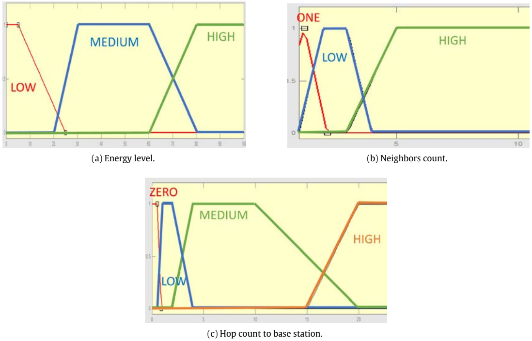
Fig. 3. Fuzzification membership functions for the three Inputs.
