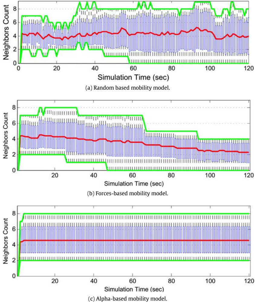
Fig. 14. Neighbors count evaluation. (For interpretation of the references to colour in this figure legend, the reader is referred to the web version of this article.)
