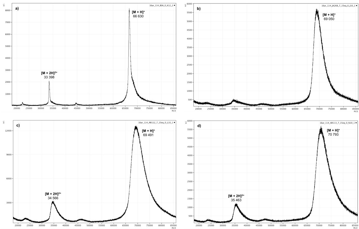
Figure 6. MALDI-TOF mass spectra of BSA (a) and fluorescent conjugates BSA-12 (b, labeling conditions: 15 eq. of NHS ester of nor -DHX-hemicyanine fused dye 12 in phosphate buffer at pH 7.0), BSA-15 (c, labeling conditions: 15 eq. of NHS ester of nor -DHX-hemicyanine fused dye 15 in phosphate buffer at pH 7.0) and BSA-18 (d, labeling conditions: 15 eq. of NHS ester of nor -DHX-hemicyanine fused dye 18 in phosphate buffer at pH 7.0) recorded in the positive mode (matrix: sinapinic acid).
