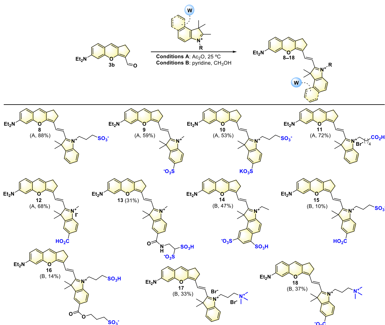
Figure 4. Synthesis of water-soluble N,N -diethylamino- nor -dihydroxanthene NIR fluorophores (compounds 13 , 15 , 16 and 18 were isolated as TFA salts; the number of TFA molecules was determined by elemental analysis).
