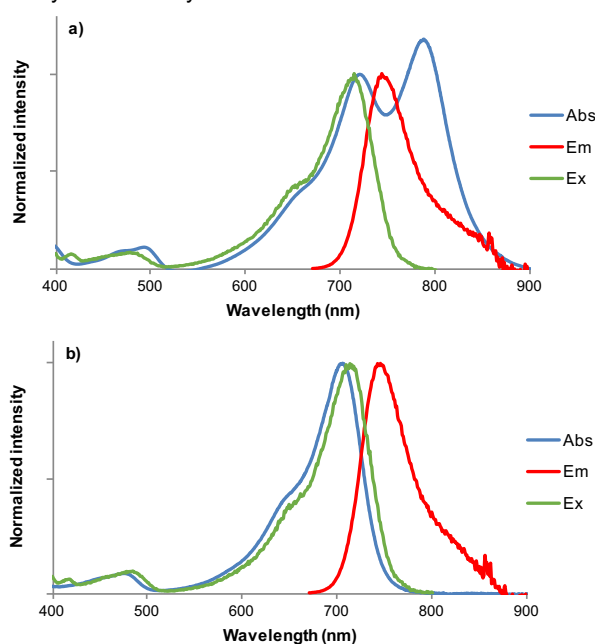
Figure 5. Normalized absorption, fluorescence emission (excitation at 650 nm) and excitation (emission at 820 nm) spectra of water-soluble N,N -diethylamino- nor -DHX NIR fluorophores 8 (a) and 17 (b) in PBS at 25 °C. Please note: absorption and fluorescence emission spectra were recorded with solutions whose concentrations are in the range 10^{-5} – 10^{-6} M and 10^{-6} – 10^{-7} M respectively. All emission spectra (also those of standard ICG) are corrected until 850 nm, which explains the artefact observed at this wavelength. If the absorption spectrum of 8 in PBS is recorded in the range of 10^{-6} – 10^{-7} M, the red-shift band at 787 nm disappears and a single maximum at 715 nm is observed.
