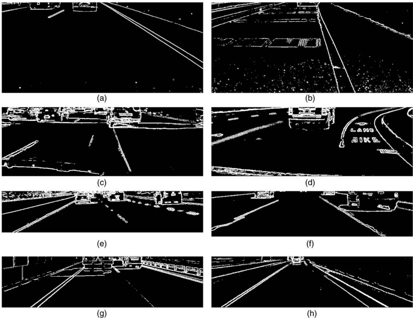
Fig. 7 Sobel edge detection with Otsu threshold: (a) multiple vehicles from the self-recorded dataset, (b) truck at lane markers from self-recorded dataset, (c) LISA-dense (frame 735), (d) LISA-urban (frame 13), (e) LISA-sunny (frame 104), (f) source-2 (frame 140), (g) iROADS-daylight, and (h) iROADS-tunnel.
