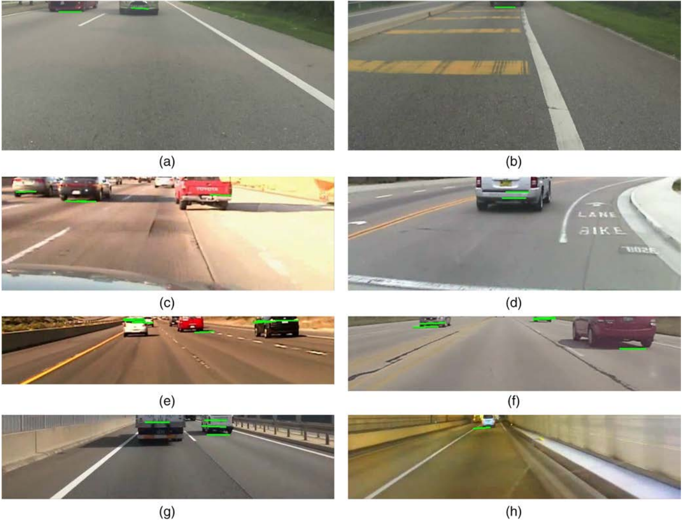
Fig. 10 Selected lines plotted on ROI images: (a) incoming vehicles from self-recorded dataset, (b) truck on lane markers from self-recorded dataset, (c) LISA-dense (frame 735), (d) LISA-urban (frame 13), (e) LISA-sunny (frame 104), (f) source-2 (frame 140), (g) iROADS-daylight, and (h) iROADS-tunnel.
