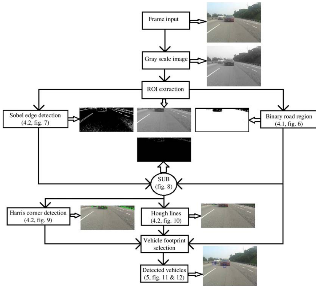
Fig. 2 Flow chart to detect the vehicles.
