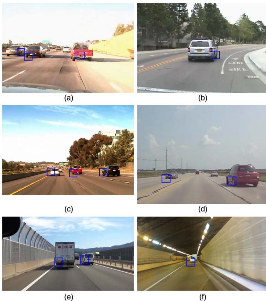
Fig. 12 Vehicle detection from online datasets: (a) LISA-dense (frame 735), (b) LISA-urban (frame 13), (c) LISA-sunny (frame 104), (d) source-2 (frame 140), (e) iROADS-daylight, and (f) iROADS-tunnel.
