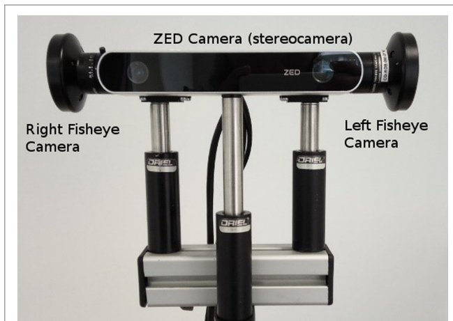
FIGURE 1 | The proposed Polydioptric Camera Rig.
