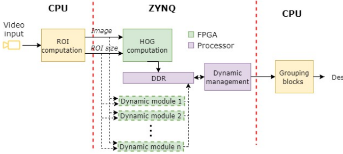
Fig. 3. Dynamic reconfigurable architecture design for pedestrian detection showing the different devices for its implementation
