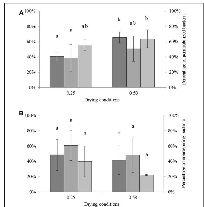
FIGURE 2 | Impact of drying on permeability and respiratory activity of Cronobacter sakazakii , Salmonella Typhimurium , and Salmonella Senftenberg cells. The number of unculturable cells was adjusted to 100% (presented on the left). (A) Impact of drying (16 h) on membrane permeability of each species reported as percentage of unculturable cells. From darker to lighter, bars represent the percentages of permeabilized C. sakazakii , S. Typhimurium , and S. Senftenberg cells (right axis). (B) Impact of drying (16 h) on respiratory activity of each species reported as percentage of unculturable cells. From darker to lighter, bars represent the percentages of non-respiring C. sakazakii , S. Typhimurium , and S. Senftenberg cells (right axis). Error bars represent the standard deviation obtained using independent triplicates.
