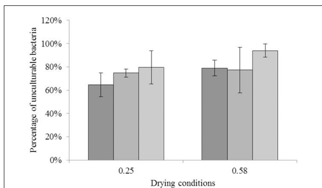
FIGURE 1 | Impact of drying on culturability. Impact of drying (16 h) on culturability of each species; the bars from darker to lighter show the percentages of unculturable Cronobacter sakazakii , Salmonella Typhimurium , and Salmonella Senftenberg cells as a function of the water activity level of drying. The equivalent logarithmic inactivation is indicated above each bar. Error bars represent the standard deviation obtained using independent triplicates. The corresponding logarithmic inactivation numbers are presented in Supplementary Table S1 .
