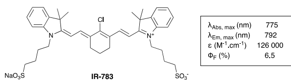
Fig. 1 Structure and main photophysical properties of the NIR-emitting cyanine dye IR-783 . \lambda_{\text{Abs,max}} , \lambda_{\text{Em,max}} and \epsilon were measured in PBS pH 7.4, at 25 °C; \Phi_{\text{F}} value in PBS pH 7.4, at 25 °C, was obtained from literature. 15
