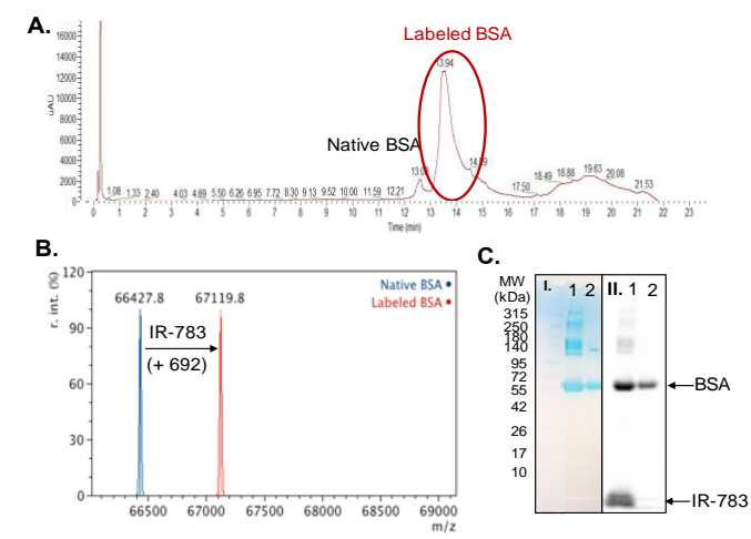
Fig. 4 (A) RP-HPLC elution profile of the purified fluorescent BSA conjugate 3 (detection at 280 nm). (B) Deconvoluted ESI-MS spectra (positive mode) of free BSA and fluorescently labelled BSA. (C) SDS-PAGE analysis of the reaction mixture (line 1) and purified fluorescent BSA conjugate 3 (line 2) after Coomassie blue staining (left panel, I.) and by fluorescence (right panel, II.) with an excitation at 740 nm and emission at 790 nm (bandwidth of 20 and 40 nm respectively).
