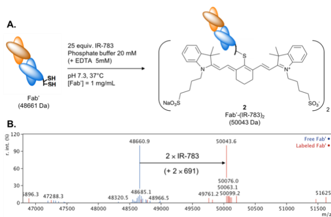
Fig. 3 (A) Labelling reaction of Fab' with IR-783 . (B) Deconvoluted ESI-MS spectra (recorded in the positive mode) of free Fab' and Fab' labelled with two IR-783 .
