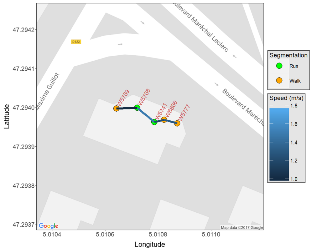
Fig. 12 Segmenting a worker trajectory in the run and walk segments to achieve semantic lines (the speed of a user is calculated in meter per second (m/s)). Value of speed is calculated between succeeding semantic locations. Based on the calculated speed values, the segments having the walk speed \leq 1.4 m/s are shown as “walk segments” in “orange” color. Whereas, the segments having the walk speed > 1.4 m/s are shown as “run segments” in “green” color
