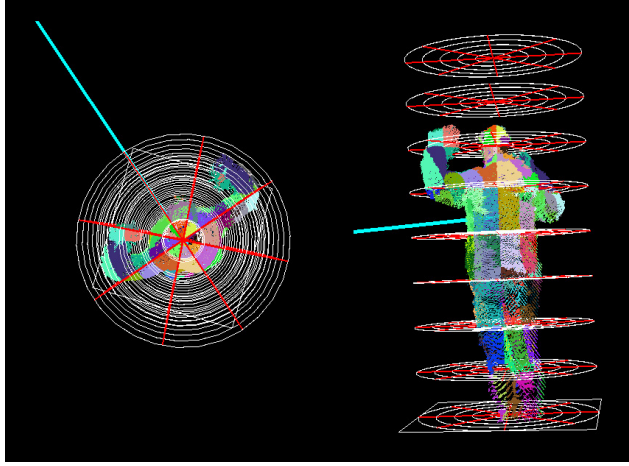
Fig. 7 Illustration of space subdivision on a CPC that represents a person. The frontal direction of the person is shown as a blue vector. a) a top view of the person shows the azimuth cut ( N_a = 8 ), the division starts at the location of the frontal vector. b) a side view of the person shows the axial cut ( N_x = 8 ) and the radial cut ( N_r = 5 ). Points in different blocks are shown in a different color.
