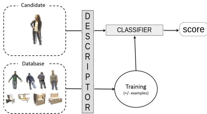
Fig. 2 Overview of the descriptor/classifier framework. The descriptor transforms the data into a more descriptive space. A classifier is built from the database of positives and negatives examples. The classifier computes for each candidate a classification score.
