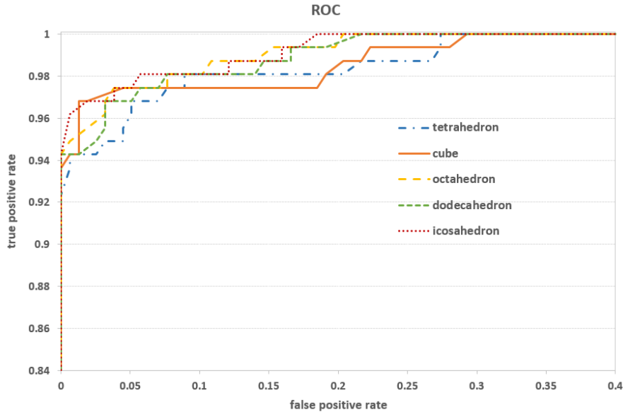
Fig. 17 ROC curves obtained with different types of polyhedrons.
