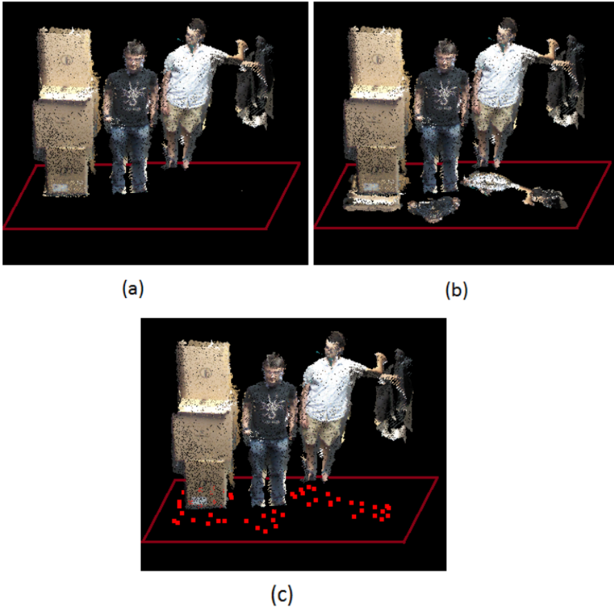
Fig. 13 CLM construction: a) CPC with the ground represented as a red rectangle, b) the projection of the CPC on the ground produces a dense point cloud, c) down-sampling of the projected cloud, the result is a set of point shown as red dots that represents the CLM.
