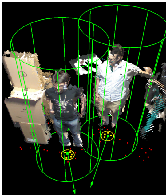
Fig. 15 Final detection results: two detected persons each marked inside a cylinder with the determined frontal vector direction (green vector).
