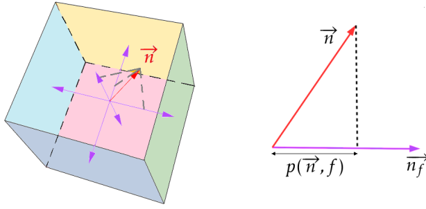
Fig. 9 Quantization of the normal vector ( \vec{n}_i ) using a cube ( n_s=6 ): a) \vec{n}_i is positioned at the center of the polyhedron to be projected on each vector \vec{g}_s that connects the center of the polyhedron and the center of its face s . b) the projection of \vec{n}_i on the vector \vec{g}_s , the result is the scalar value \hat{q}_{i,s} .
