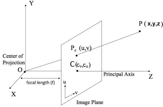
Fig. 4 Illustration of the pin-hole camera model.
