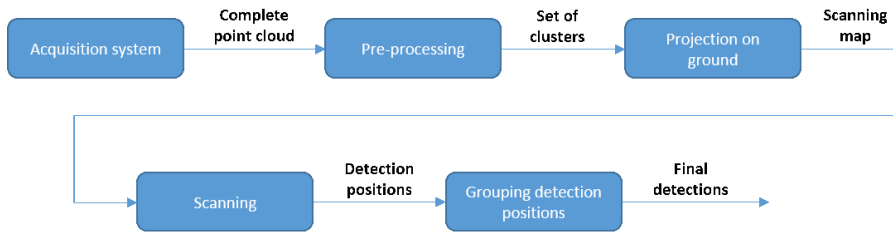
Fig. 11 Human detection procedure pipeline.
