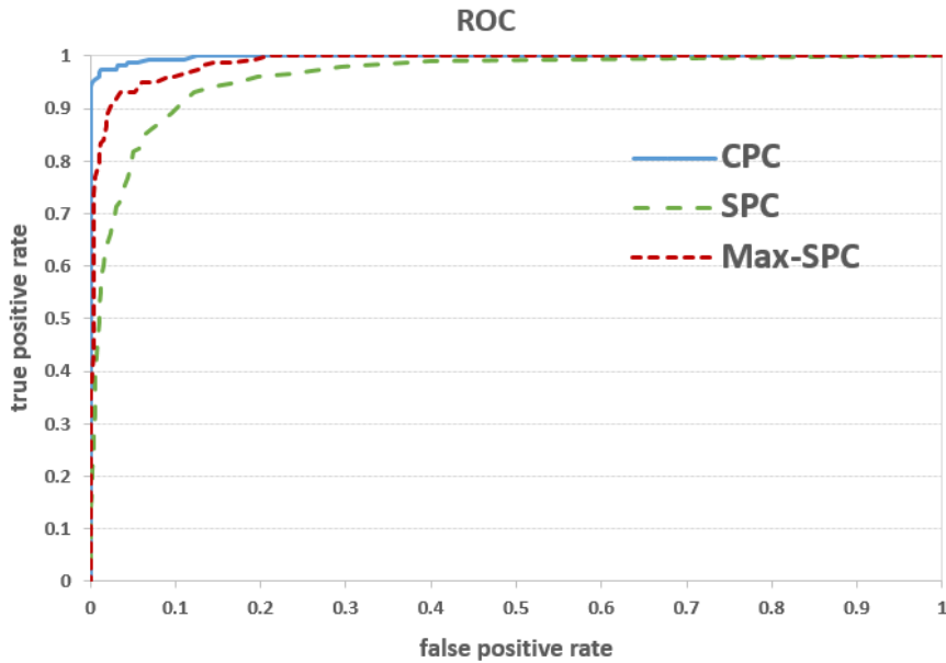
Fig. 20 ROC curves obtained from our complete point cloud (CPC) and with the point cloud of each kinect taken individually (SPC) or combined (Max-SPC). A single view decreases significantly the performances and our CPC outperforms the combination of single point cloud.
