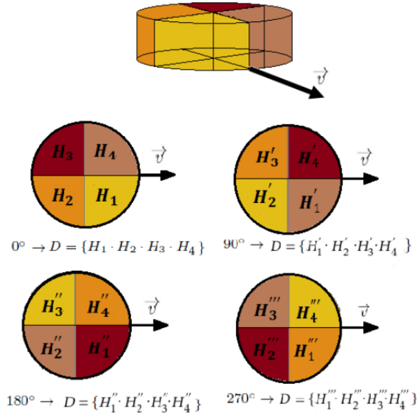
Fig. 19 Descriptor construction relative to the frontal orientation vector \vec{v} : (top) cylinder division into blocks; (down) each rotation of the frontal vector yields a new descriptor.
