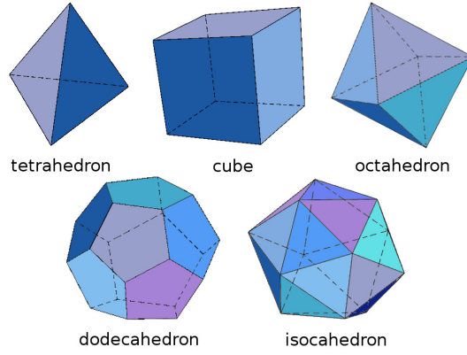
Fig. 8 The five regular polyhedrons.
