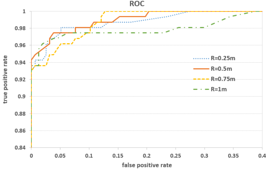
Fig. 16 ROC curves obtained with different values of cylinder radius.
