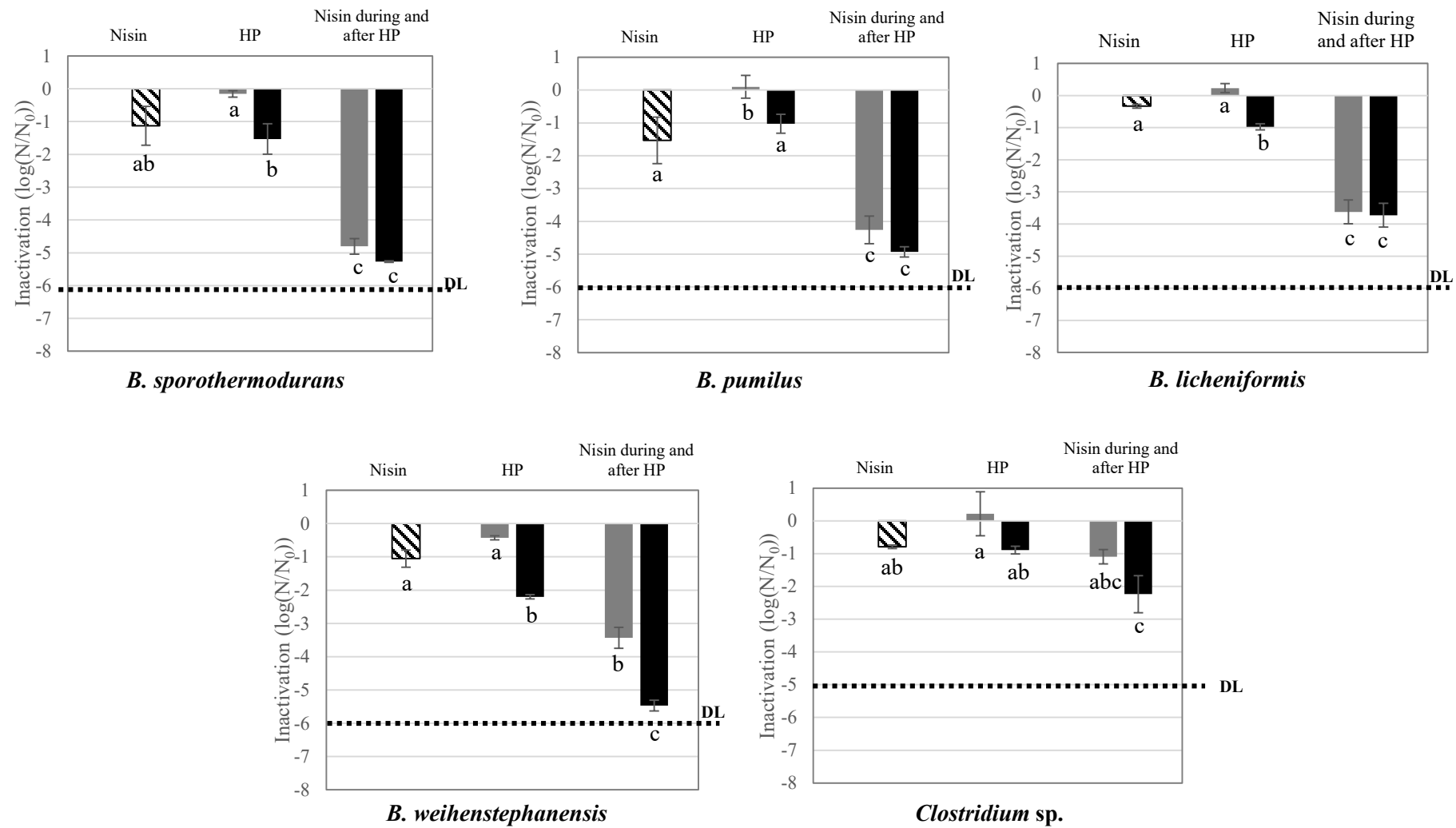
Fig 2. Effect of nisin addition on high pressure inactivation of spores (500 MPa, 10 min). Treatment in nutrient media. Spores of B. weihenstephanensis and Clostridium sp. were treated in MMH; spores of B. sporothermodurans ; B. pumilus and B. licheniformis were treated in milk. Nisin concentrations: 50 IU/mL for Bacillus spp. 20 IU/mL for Clostridium sp. Striped bars: effect of nisin alone; Grey bars: effect of HP treatment at 20 °C; Black bars: effect of HP treatment at 50 °C. DL: Detection limit. Error bars represent SD calculated from independent triplicates. The letters represent a significant difference ( p < 0.05 ) obtained with Tukey's HSD (Honest Significant Difference) test.
