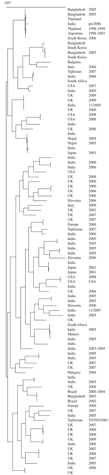
Fig. 6. Dendrogram (Maximum Parsimony) of sequences of the gene encoding VP7 of G12 strains. Strains included are global and represent introductions between 1991 and 2009.
