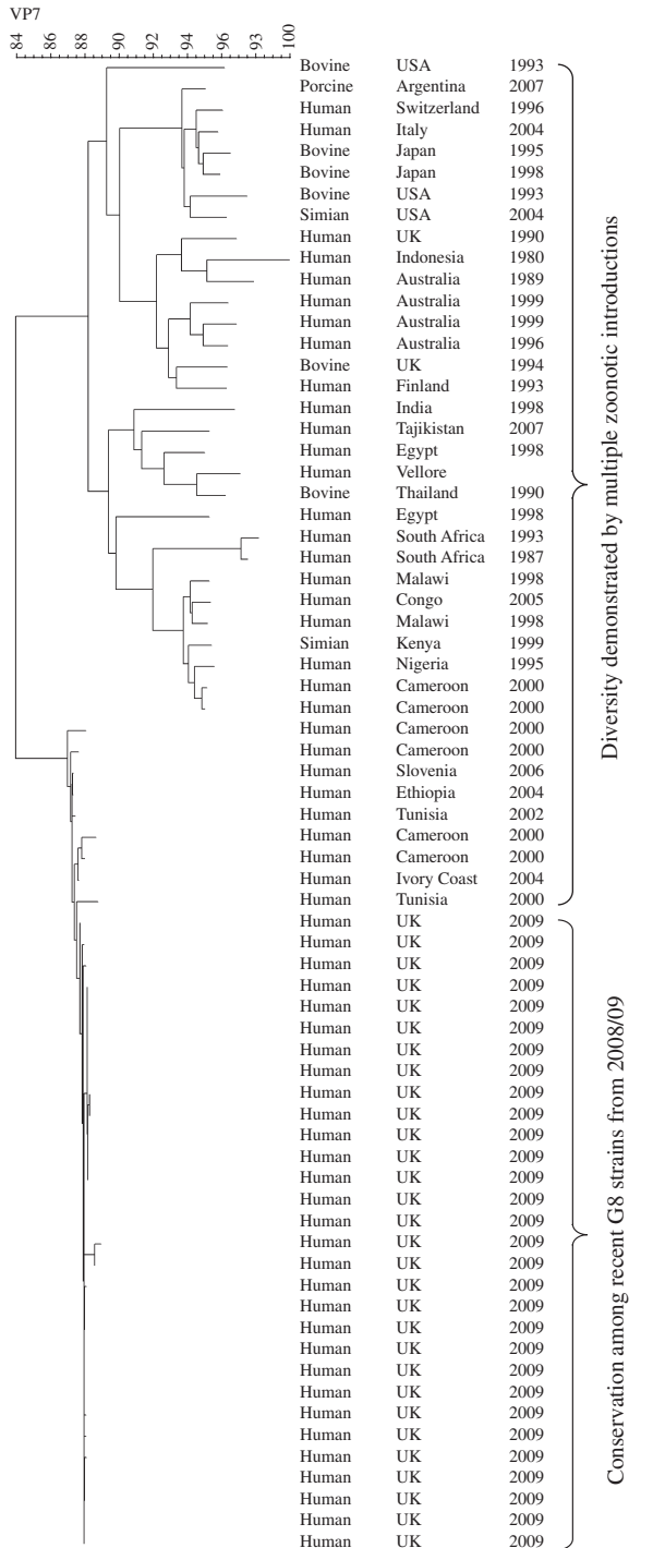
Fig. 5. Dendrogram (Neighbour Joining) of sequences of the gene encoding VP7 of G8 strains. Host, country and year of identification are indicated after each strain.
