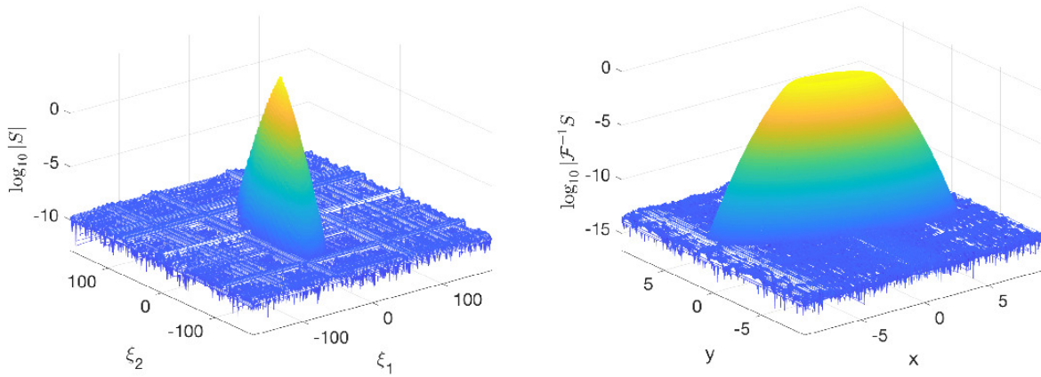
FIGURE 8. Solution S to the equation (13) for the asymmetric potential for k = 0 and \epsilon = 1/128 on the left and its inverse Fourier transform on the right.
