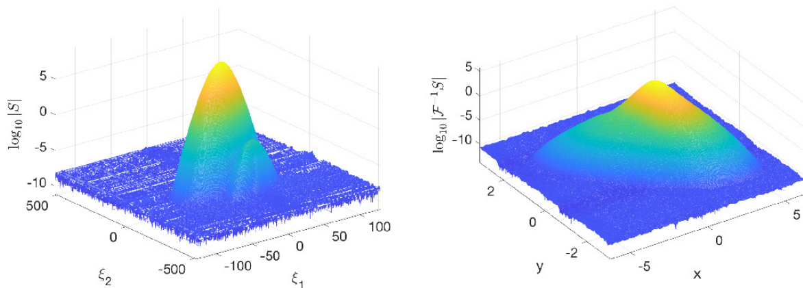
FIGURE 10. Solution to the S equation (13) for the asymmetric potential for k = 1 and \epsilon = 1/128 on the left, and its inverse Fourier transform on the right.
