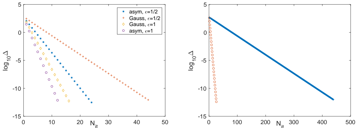
FIGURE 2. The quantity \Delta = \|S^{(n+1)} - S^{(n)}\|_\infty in a logarithmic plot for the iterative solution of (22) for the Gaussian and asymmetric potentials for k = 0 and \epsilon = 1, 1/2 in dependence of the number of iterations N_{it} on the left; on the right the same quantity for the asymmetric potential, \epsilon = 1/4 and k = 0 ('+') and k = 1 ('o').
