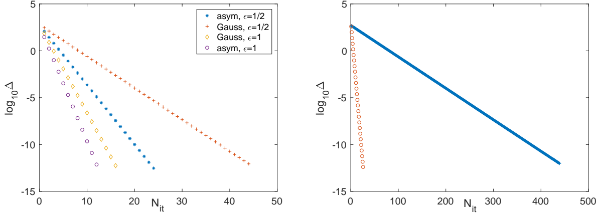
FIGURE 2. The quantity \Delta = \|S^{(n+1)} - S^{(n)}\|_\infty in a logarithmic plot for the iterative solution of (22) for the Gaussian and asymmetric potentials for k = 0 and \epsilon = 1, 1/2 in dependence of the number of iterations N_{it} on the left; on the right the same quantity for the asymmetric potential, \epsilon = 1/4 and k = 0 ('+') and k = 1 ('o').
