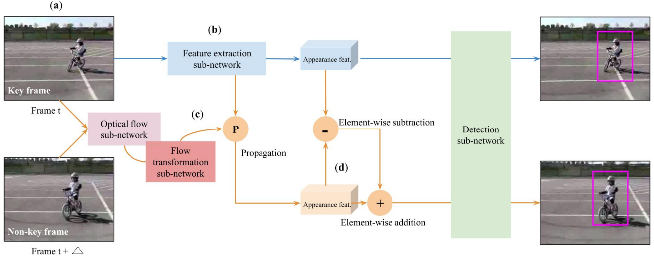
Figure 1: Illustration of our motion-guided action detection framework with motion-aware appearance features. (a) Two types of input frames. (b) For a key frame, appearance feature is obtained from the CNN feature extraction sub-network. (c) For a non-key frame, the flow sub-network estimates a flow field between the non-key frame and its preceding key frame. The resulted flow is first transformed and then used to propagate appearance feature. (d) An implicit motion cue (difference in features) amplifies the appearance feature. Blue and orange arrows are carried out at a key and non-key frame respectively.
