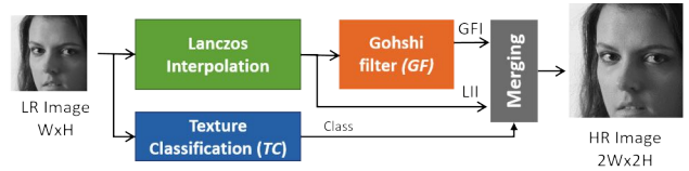
Fig. 5 LASSR method
