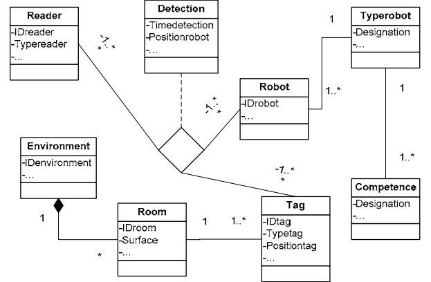
Fig. 5. Class diagram of the proposed centralized database
