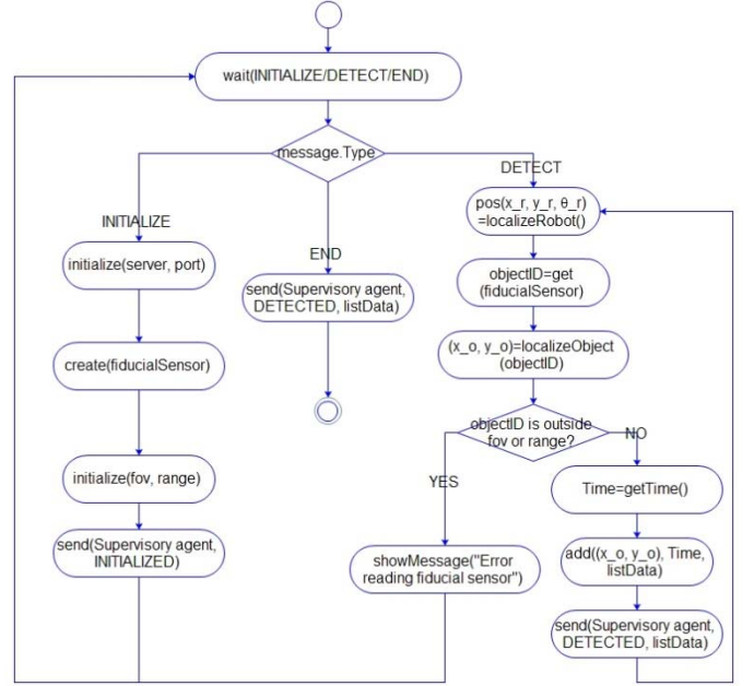
Fig. 4. Behavior diagram of the Robot agent . initialize(field 1 ... field n ) initializes field 1 ... field n of the Robot agent . create(sensor) creates a sensor to equip the mobile robot. localizeRobot() returns the actual position ( x, y, \theta ) of the mobile robot. add( v_1, \dots, v_n , listData) adds v_1, \dots, v_n to listData . localizeObject(ID) localizes the object with ID into the workspace of the robot. getTime() gets the current time when the object is detected.
