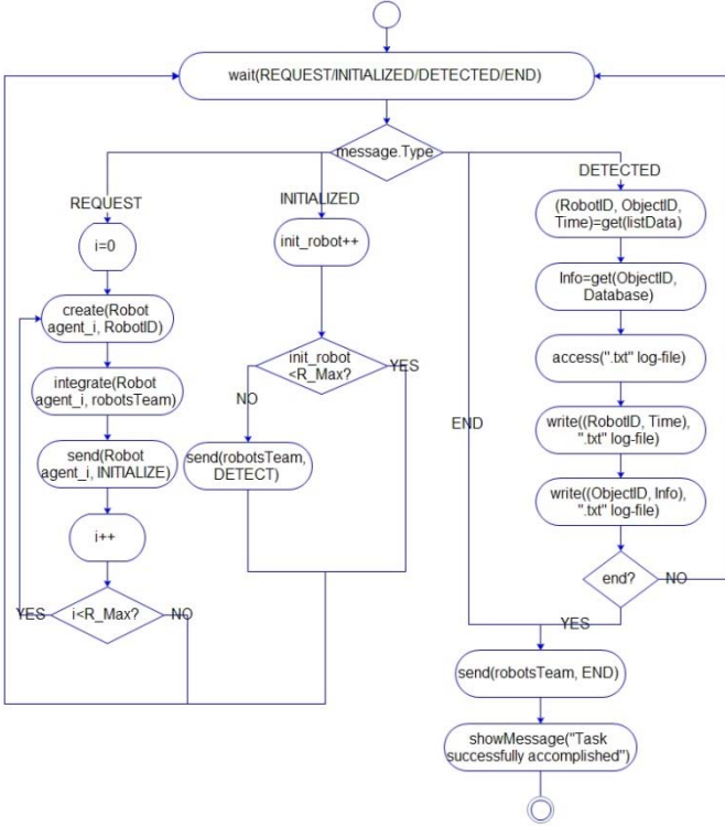
Fig. 3. Behavior diagram of the Supervisory agent . create(Agent, ID) creates an Agent with ID to locally control a mobile robot. integrate(Agent, Team) integrates a new Agent into the Team . send(Agent, Message) sends Message to Agent . get(listData) receives listData from the operator, another agent, a sensor equipping a robot or from the knowledge database. access(File) blocks the execution until getting rights to access File . write( v_1, \dots, v_n , File) writes v_1, \dots, v_n into File . showMessage(Message) displays Message on the screen of the human operator.
