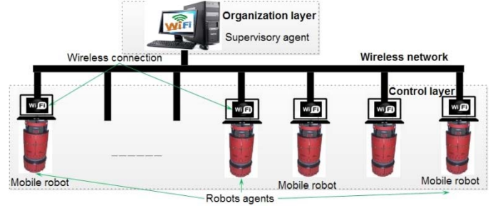
Fig. 2. The distributed multi-agent control architecture for RFID CPRS
