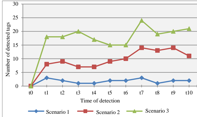
Fig. 7. Comparison between the obtained results for tags detection and identification
