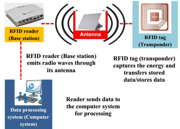
Fig. 1. Principle of RFID technology
