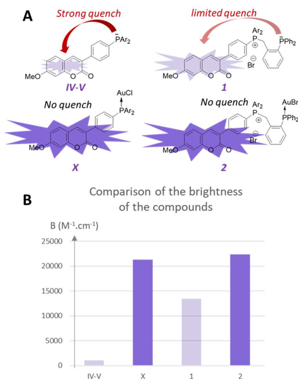
Figure 3. Explanation of the difference of quench phenomenon intensity for the different compounds (top) and its impact on the brightness (brightness, B = \epsilon\Phi_f ) of the corresponding compounds (bottom).
