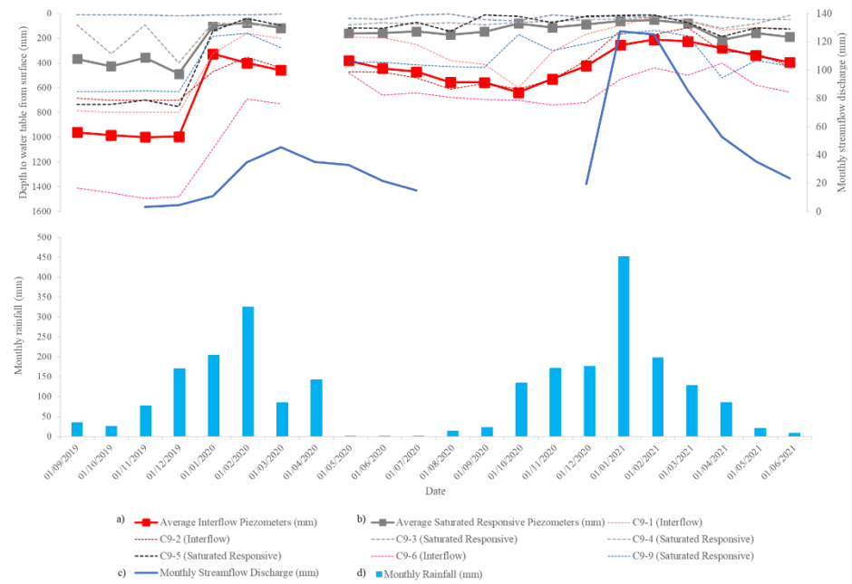
Figure 8. Comparisons of piezometer data installed in the (a) interflow soils, (b) saturated responsive soils, (c) monthly streamflow discharge and (d) monthly rainfall in CP-IX.
