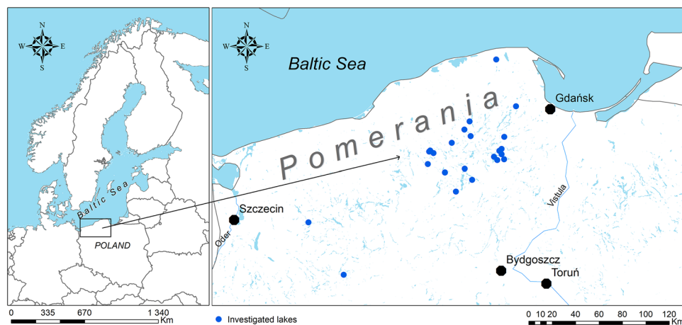
Fig. 1 Localization of the investigated lakes
