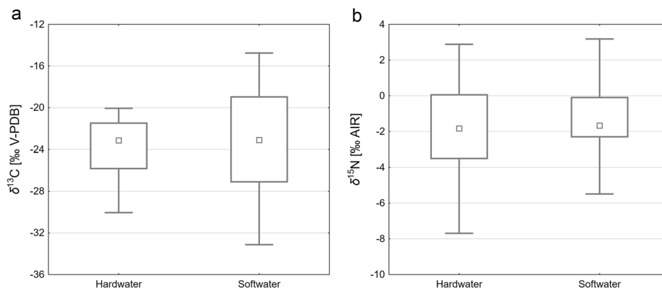
Fig. 2 Comparison of N. flexilis in hardwater ( N=12 ) and softwater ( N=11 ) lakes: a \delta^{13}\text{C} values; b \delta^{15}\text{N} values. Median, box 25–75% and min–max. Mann–Whitney U test: p > 0.05 in both cases
