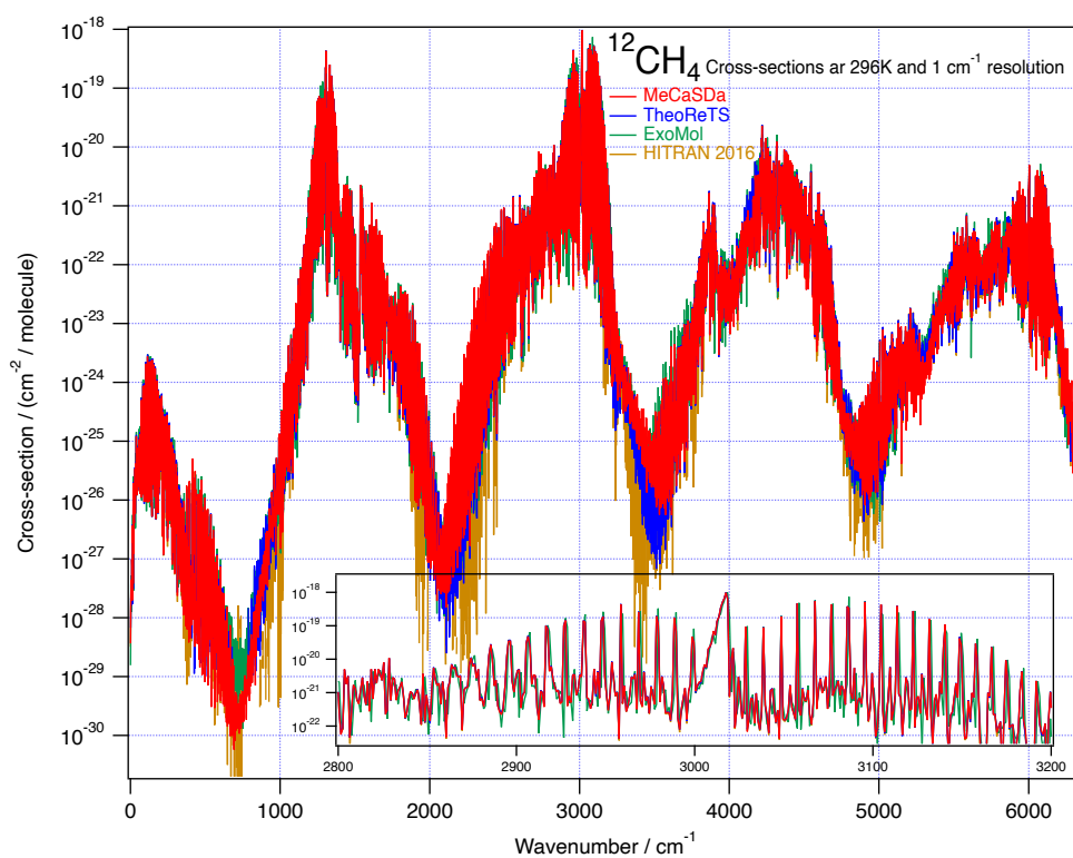
Figure 2: Calculated cross-sections (logarithmic scale) at a temperature of 296 K and a resolution of 1 \text{ cm}^{-1} for the ^{12}\text{CH}_4 molecule. Data are compared to ExoMol (green curve), TheoReTS (blue curve) and HITRAN 2016 (brown curve) showing a good match except in the 800 \text{ cm}^{-1} region where a lack of hot bands and high J value data explain these discrepancies. The insert shows the region of the \nu_3 stretching fundamental.
