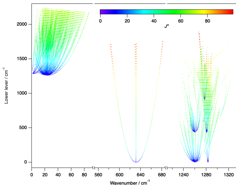
Figure 6: Representation of the lower level wavenumber for all transitions present in the TFMeCaSDa database. Colors are used to display the lower state rotational quantum number value, J'' .
