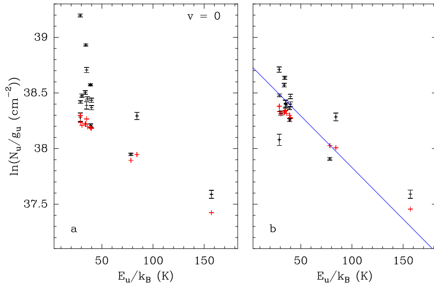
Figure 4: Population diagram of NH 2 CH 2 CN, v = 0 toward Sgr B2(N2). The observed datapoints are shown in black while the synthetic populations are shown in red. No correction is applied in panel a . In panel b , the optical depth correction has been applied to both the observed and synthetic populations and the contamination by all other species included in the full model has been removed from the observed datapoints. The blue line is a linear fit to the observed populations (in linear-logarithmic space).
