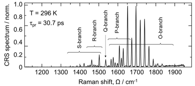
FIG. 4. Single-shot CH 4 \nu_2 CSRS spectrum at room-temperature. The \nu_2 mode Raman-activity is completely anisotropic and the selection rules allow for O-, P-, Q-, R-, and S-branch transitions. Note that, as the CRS signal is acquired in the Stokes side, the usual branch ordering is reverted, with negative changes in the total angular momentum quantum number ( \Delta J=-1, -2 for the P- and O-branch, respectively) determining a larger frequency transition.
