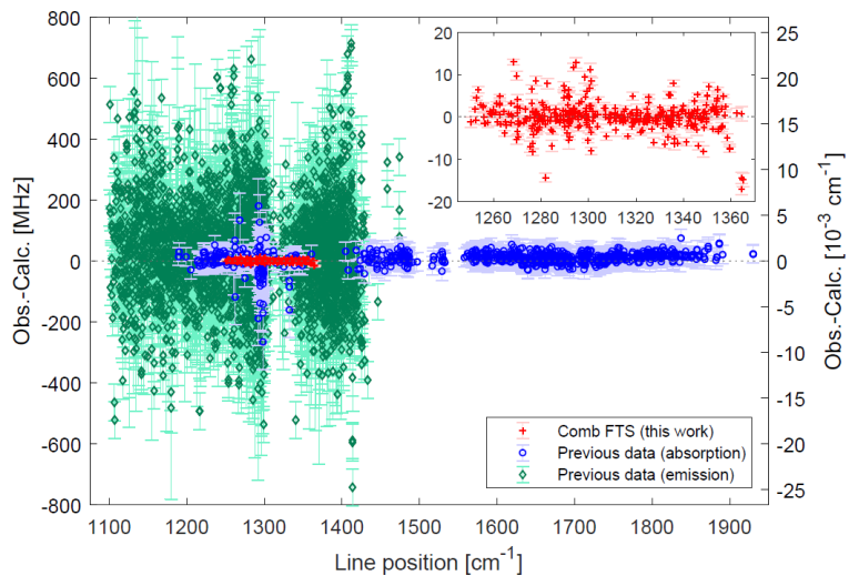
Figure 4. The residuals of the global fit for the ^{12}\text{CH}_4 P_2-P_1 line positions from optical frequency comb FTS absorption measurements reported in this work ( 2\nu_4 - \nu_4 and \nu_2 + \nu_4 - \nu_2 bands, red crosses) as well as from previous absorption (blue circles) and emission (green diamonds) spectroscopy studies [25]. Inset: detailed view of the spectral lines reported in this work.
