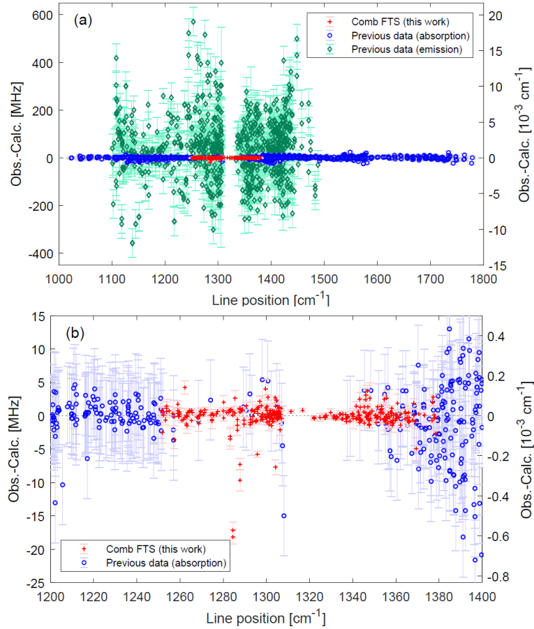
Figure 3. (a) The residuals of the global fit for the ^{12}\text{CH}_4 P_1-P_0 line positions obtained from optical frequency comb FTS absorption measurements reported in this work ( \nu_4 band, red crosses) as well as from previous absorption (blue circles) and emission (green diamonds) spectroscopy studies [25]. (b) Detailed view of the spectral range including the lines reported in this work. The reduced uncertainty of the comb FTS measurements as compared to previous absorption measurements is evident. (For clarity, previous emission measurements are not shown.)
