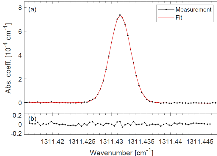
Figure 2. (a) Absorption spectrum of the (J,C,a): (1, A_2, 1) \leftarrow (0, A_1, 1) line of the ^{12}\text{CH}_4 v_4 band at a concentration of 5% and a total pressure of 0.04 mbar (black markers) together with a fitted Voigt line profile (red line). (b) Fit residuals.
