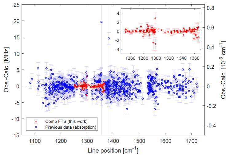
Figure 5. The residuals of the global fit for the ^{13}\text{CH}_4 P_1 - P_0 line positions from optical frequency comb FTS absorption measurements reported in this work ( \nu_4 band, red crosses) as well as from previous absorption measurements (blue circles) [23]. Inset: detailed view of the spectral lines reported in this work
