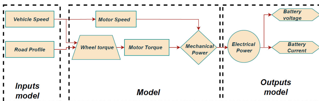
Figure 4. Electric model of METALLIANCE's MSV machine.
