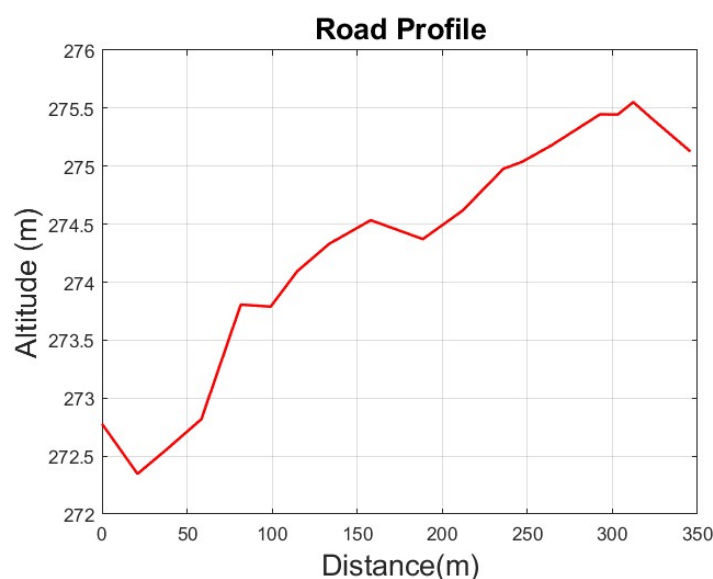
Figure 3. Road profile of the METALLIANCE test site (altitude vs distance).
