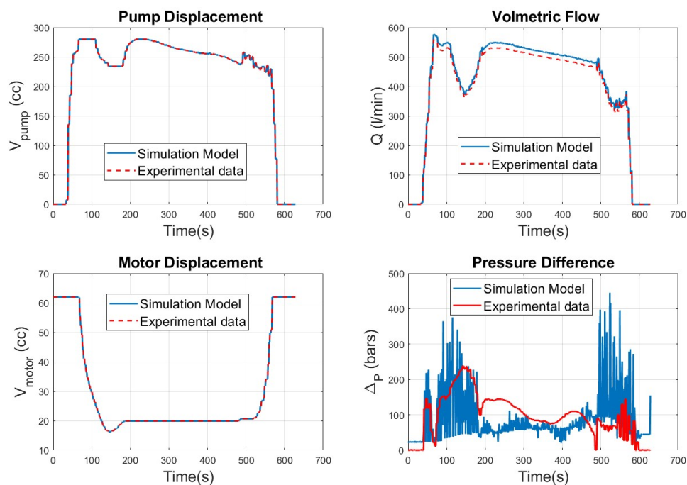
Figure 10. Comparison of simulation results with recorded data of pump and motor displacement, volumetric flow, and pressure difference.
