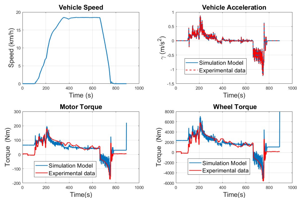
Figure 5. Vehicle speed profile, comparison of simulation results with recorded data of vehicle acceleration, motor, and wheel torque.
