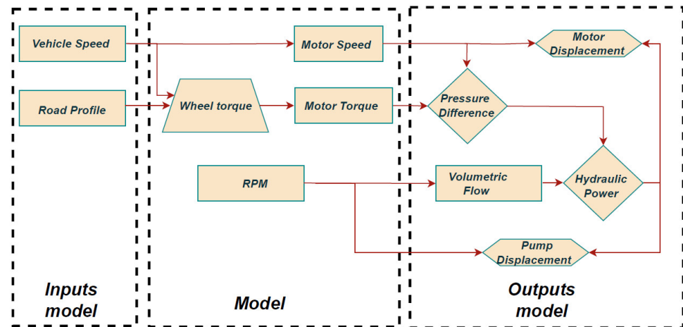
Figure 8. Simulink hydraulic model of METALLIANCE's MSV machine.
