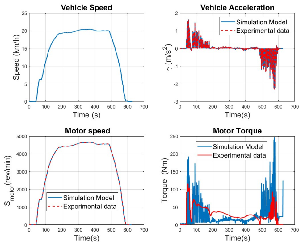
Figure 9. Comparison of simulation results with recorded data of vehicle speed and acceleration, motor torque, and speed.
