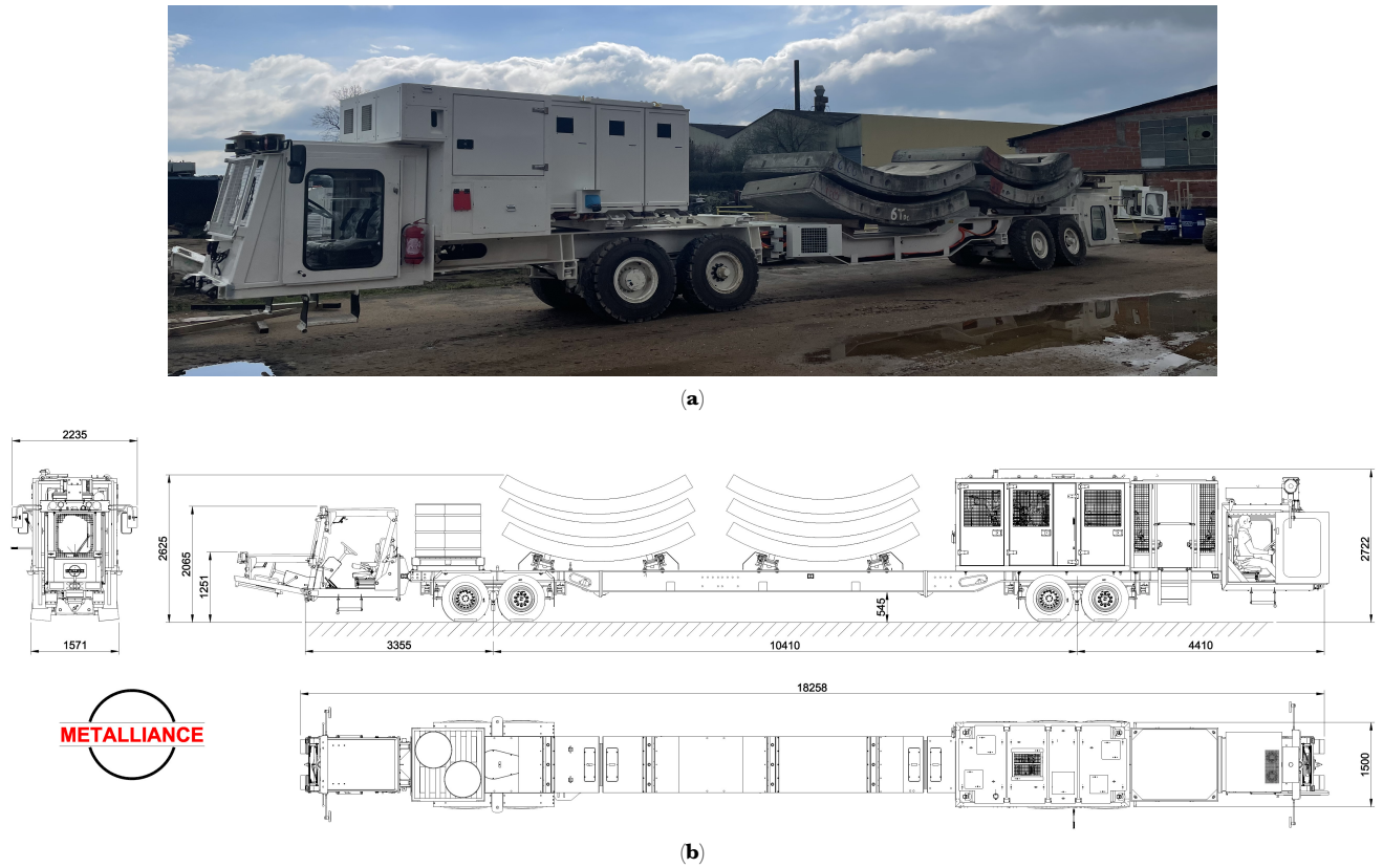
Figure 1. (a) A real METALLIANCE's multi-service vehicle (MSV); (b) Schematic Diagram of the METALLIANCE's MSV.
