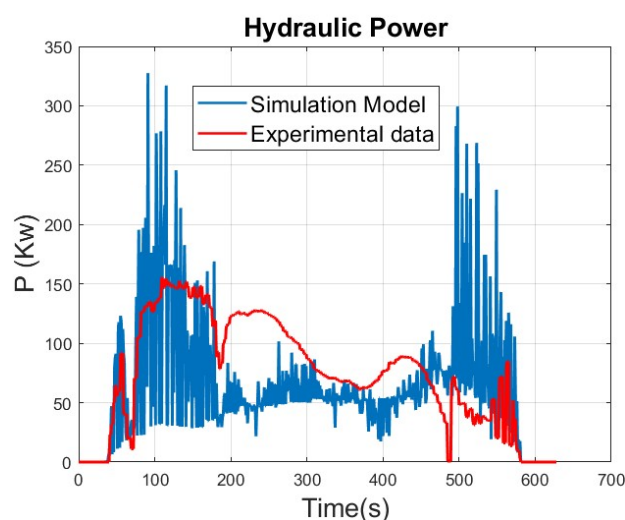
Figure 11. Comparison of simulation results with recorded data of hydraulic power.
