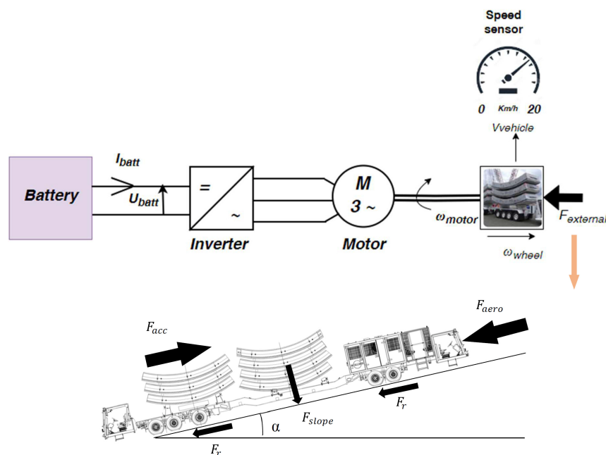
Figure 2. Schematic of the vehicle drive system and external forces acting on the vehicle moving.
