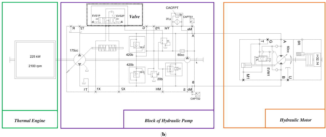
Figure 7. (a) General hydrostatic transmission structure (from the engine to drive wheels); (b) schematic of hydrostatic transmission with ISO symbol; (c) real hydrostatic transmission circuit for METALLIANCE's machine.
