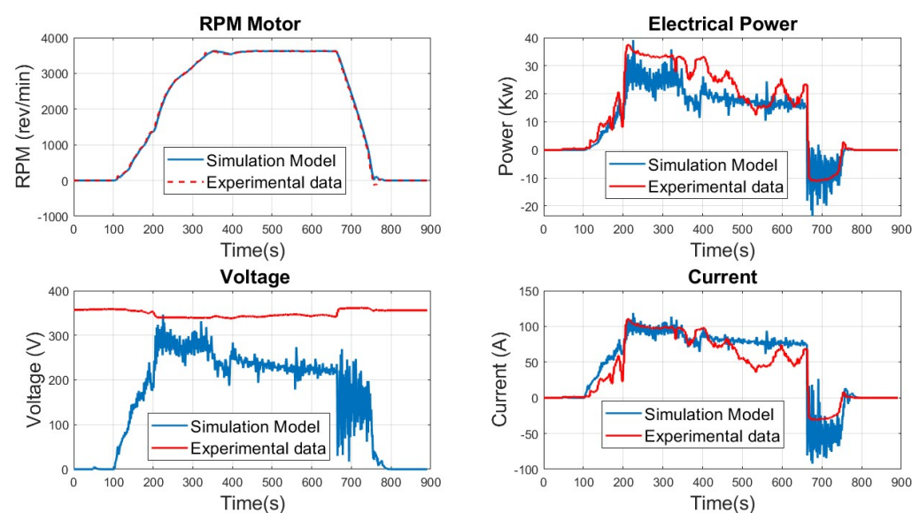
Figure 6. Comparison of simulation results with recorded data of motor speed, electrical power, battery voltage, and current.
