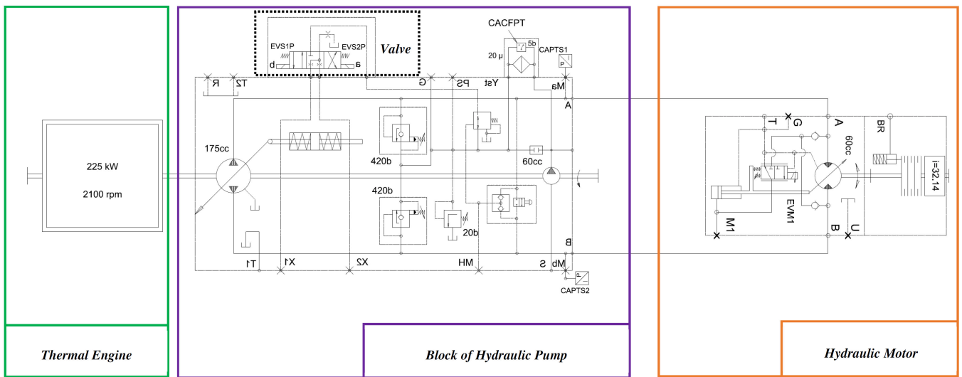
Figure 7. (a) General hydrostatic transmission structure (from the engine to drive wheels); (b) schematic of hydrostatic transmission with ISO symbol; (c) real hydrostatic transmission circuit for METALLIANCE's machine.
