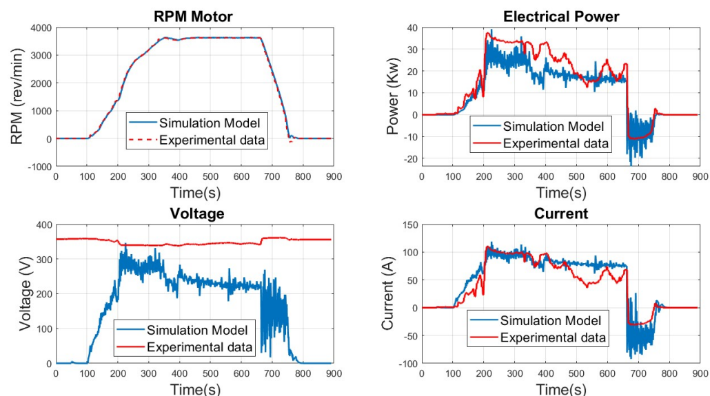
Figure 6. Comparison of simulation results with recorded data of motor speed, electrical power, battery voltage, and current.
