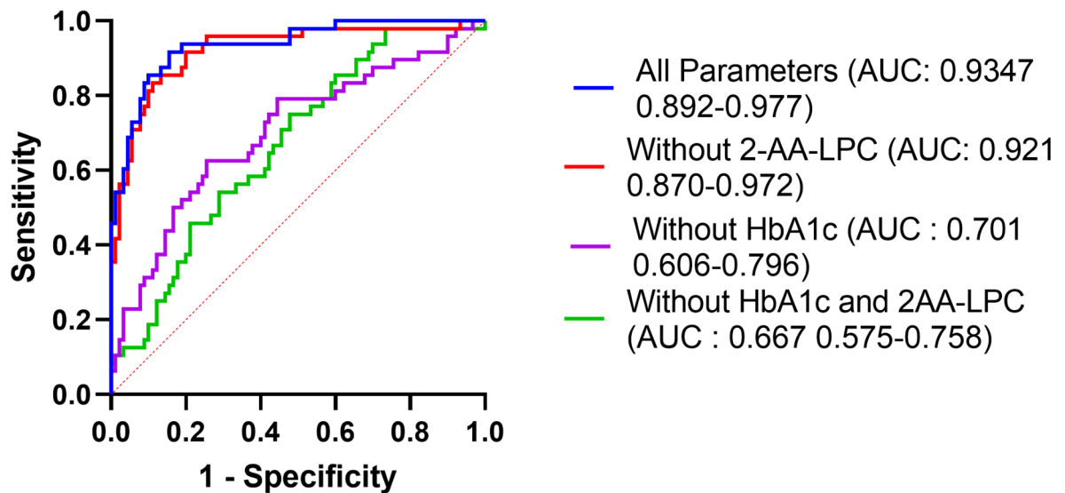
Fig. 2 A: Forest plots showing odds ratio values and 95% confidence intervals for multivariable logistic regression analysis of diabetes and biological variables. B: Receiver operating characteristic curve (ROC) for the prediction of type 2 diabetes based on the selected biological parameters. (AUC: Area under the Curve)
