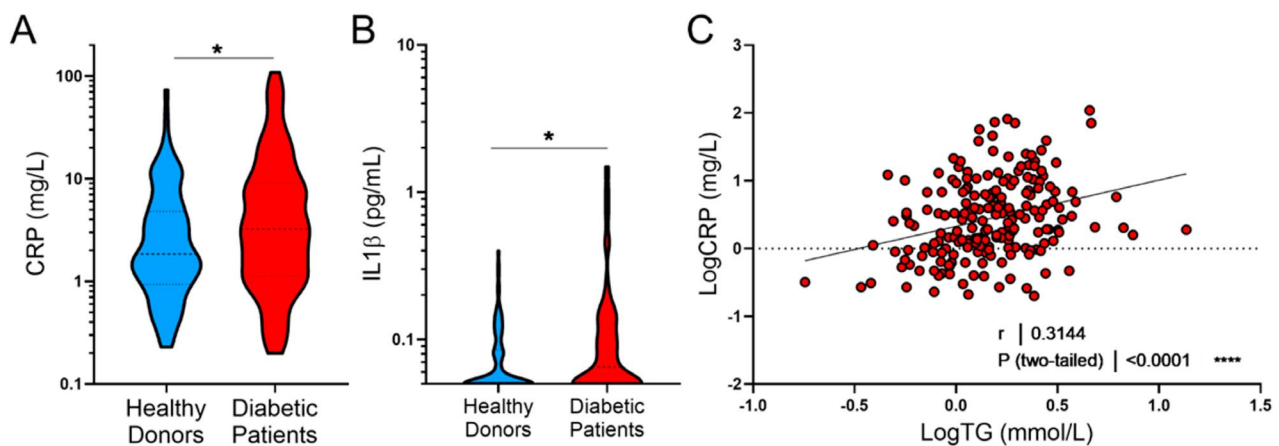
Fig. 1 A: Violin plot of C-reactive protein (CRP) levels in control and T2DM patients. B: Violin plot of IL-1 \beta levels in control and T2DM patients. C: Correlation between plasma HsCRP levels and triglycerides (R and P values were obtained by the Spearman rank test)
