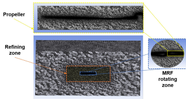
FIGURE 8 Elements of the entire, refining, and propeller fluid domains.
