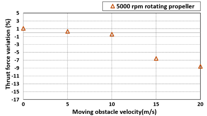
FIGURE 15 Effect of moving obstacle proximity (0.2m) on the propeller thrust (5000 rpm).
