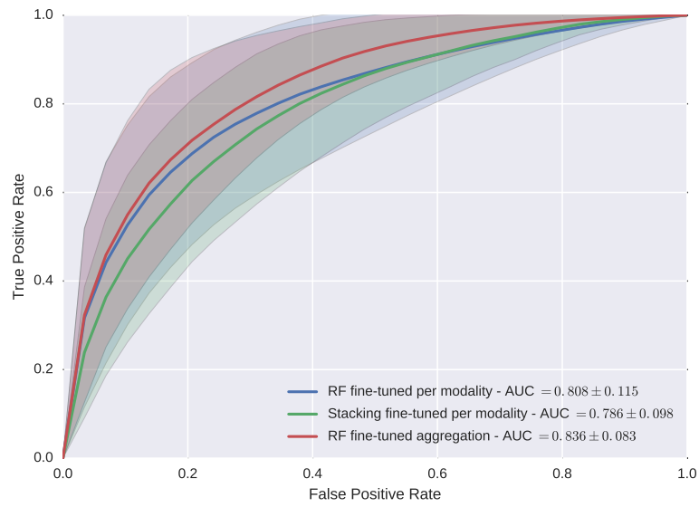
Figure 6.9: Analysis of feature combination approaches after fine tuning through balancing and feature selection/extraction.
