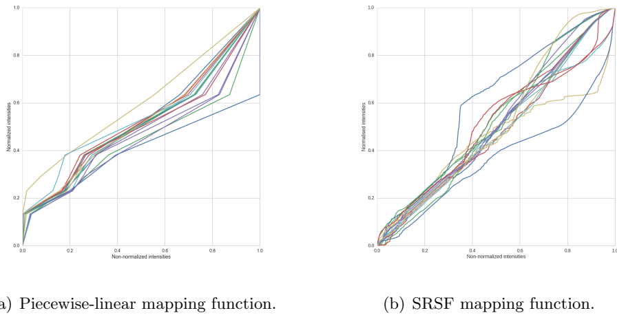
Figure 5.2: Comparison of the mapping functions found with the piecewise-linear and SRSF-based normalization. Each curve corresponds to a mapping function for a single patient.
