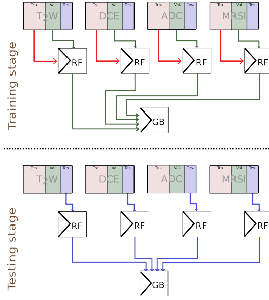
Figure 6.4: The principle of stacking. First, training samples (red) are used to train each individual RF. Subsequently, a validation set (green) is provided to each RF which outputs a set of probabilities used for the classification of the meta-classifier. Finally, a test set is used to assess the classification performance to whole stack.
