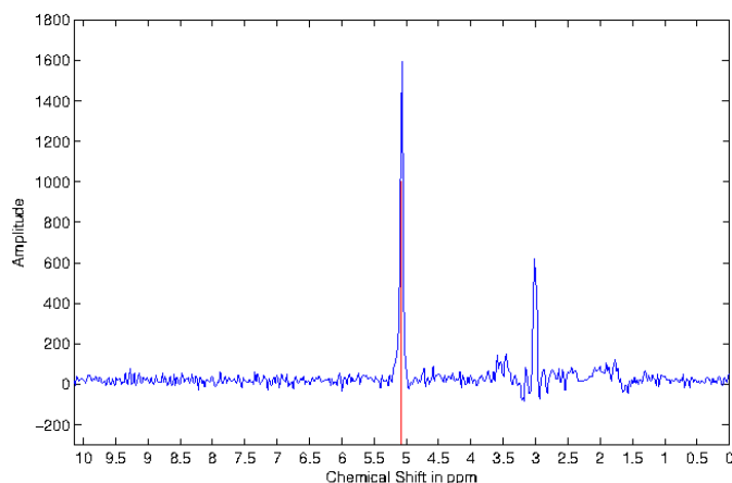
Figure 3.8: Illustration of frequency misalignment in a MRSI spectra acquired with a 3 T MRSI scanner. The water peak is known to be aligned at 4.65 ppm. However, it can be seen that the peak on this spectra is aligned at around 5.1 ppm.
